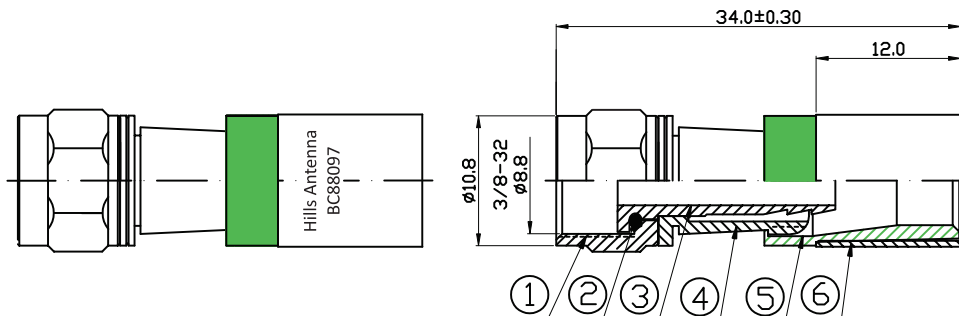
Schematic Diagram
